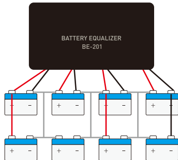
Figure 2: Multiples sets of batteriaes
