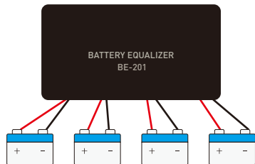
Figure 1: 4* 12V battery bank
